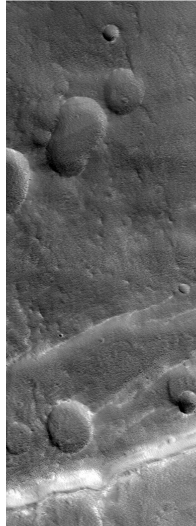
Figure 7: Ambiguous features on the flank of Pavonis Mons. Are these craters or subsidences created by collapsed lava tubes? Image credit MGS MOC.
