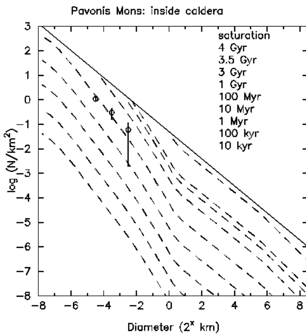
Figure 5: Isochron chart for Pavonis Mons, caldera.
